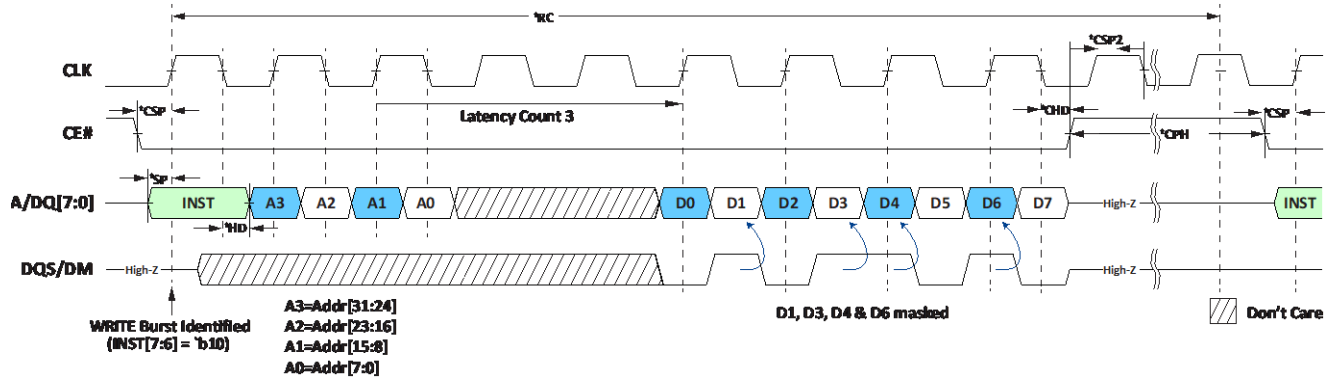
Figure 10: Synchronous Write followed by any Operation
